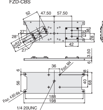
3D Camera Base FZD-CBS
