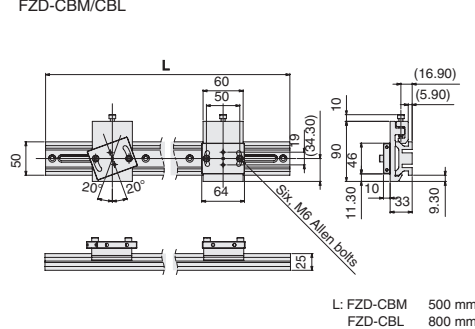
3D Camera Base FZD-CBM/CBL
