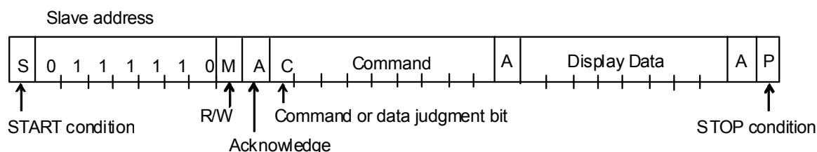
Figure 8. Interface protocol
