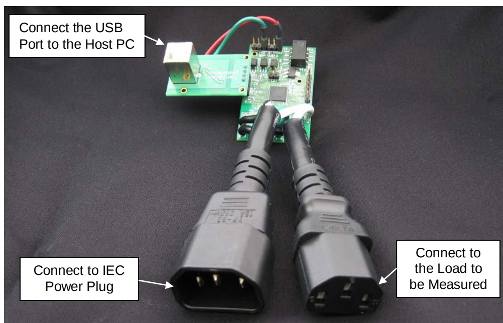
Figure 1: AC-PMON Connections
