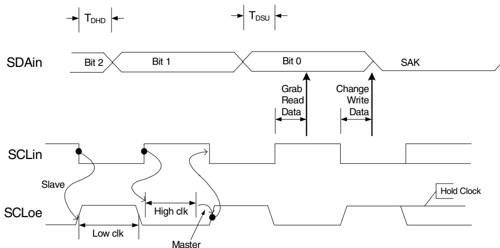
Figure 25-3. I 2 C Data and Clock Timing Generation
