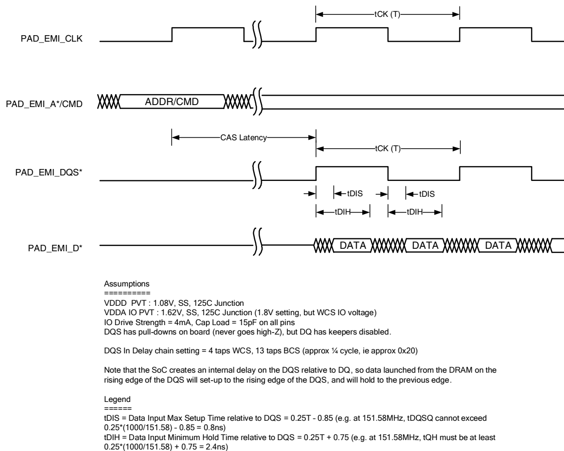
Figure 2-4. i.MX23 EMI mDDR DRAM Input AC Timing
