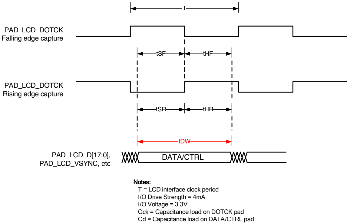
Figure 2-7. LCD AC Output Timing Digram
