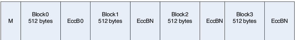
Figure 35-11. Valid layout for 2112 bytes sized page
