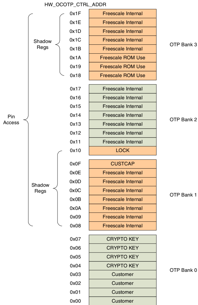
Figure 7-2. OCOTP Allocation
