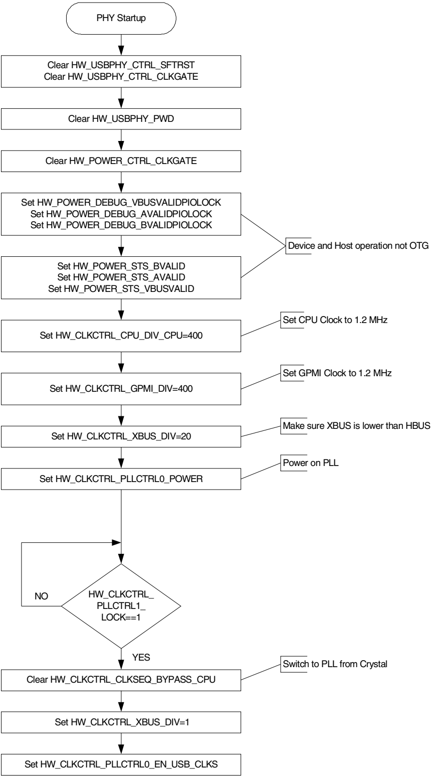
Figure 8-3. USB 2.0 USB PHY Startup Flowchart
