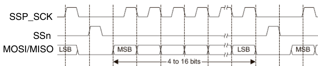
Figure 21-3. Motorola SPI Frame Format with POLARITY=0 and PHASE=0
