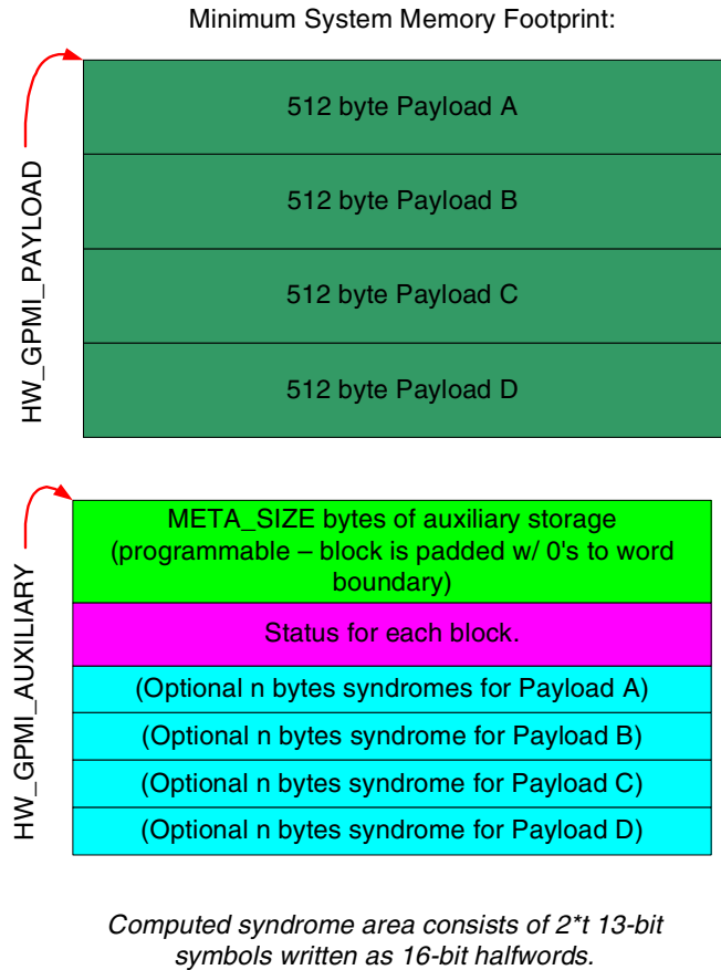
Figure 15-4. BCH Data Buffers in Memory
