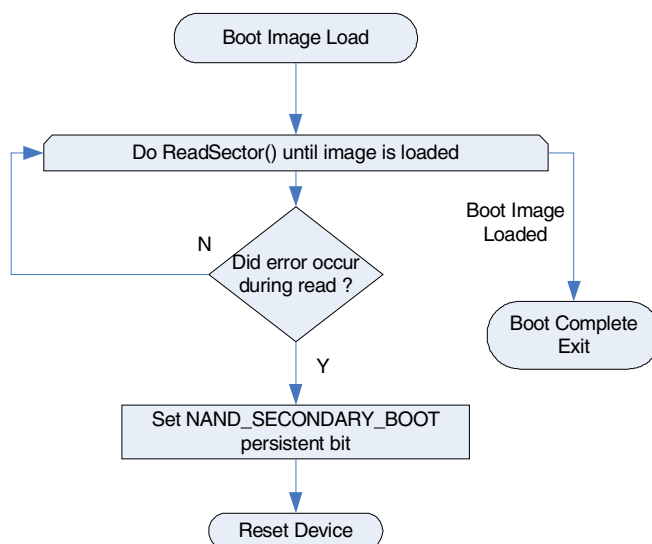
Figure 35-8. Boot Image Recovery
