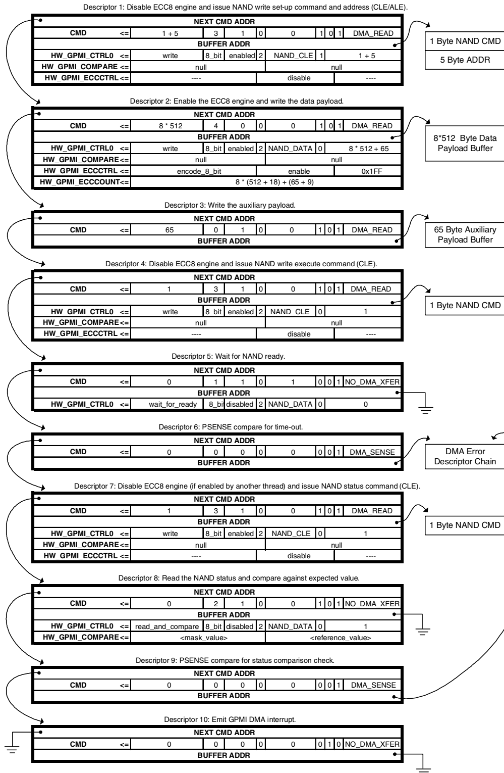
Figure 14-8. ECC8 Reed-Solomon Encode DMA Descriptor Chain
