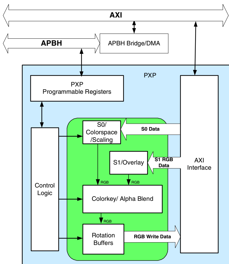
Figure 17-1. Pixel Pipeline (PXP) Block Diagram
