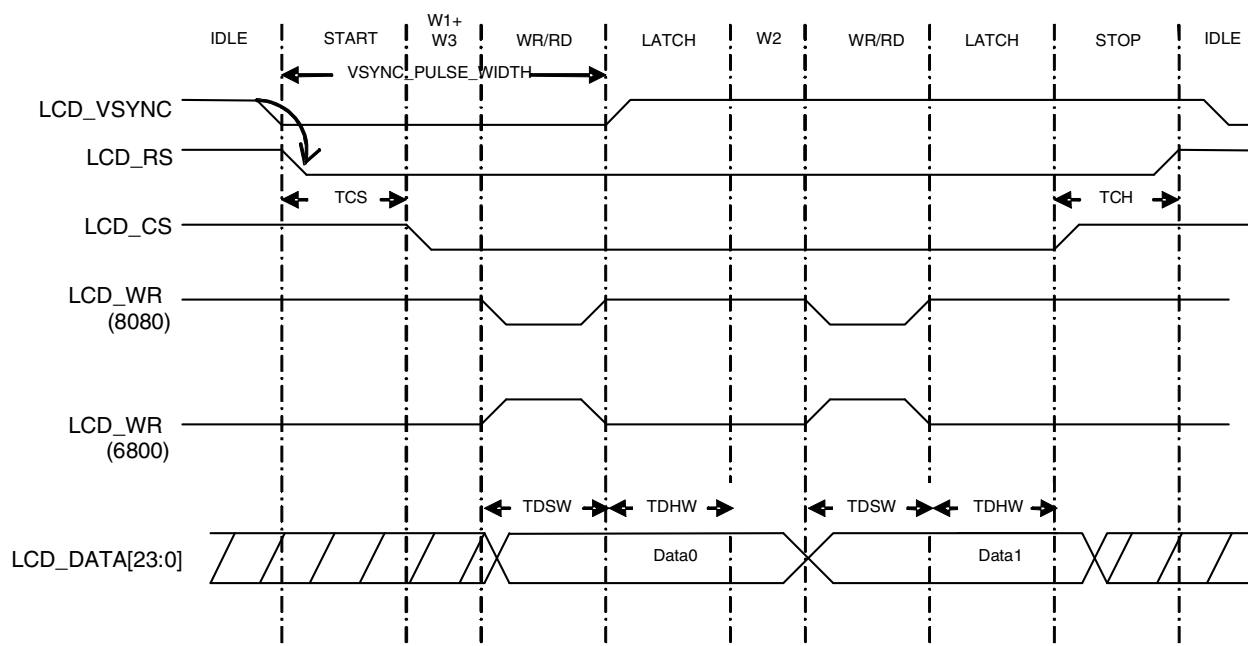
Figure 18-7. LCD Interface Signals in System Write Mode
