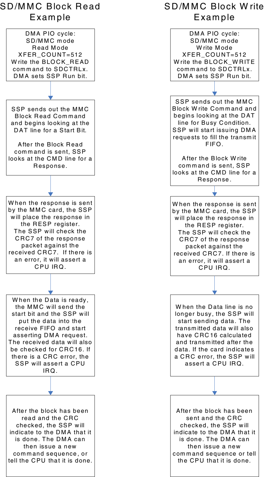
Figure 21-11. SD/MMC Block Transfer Flowchart
