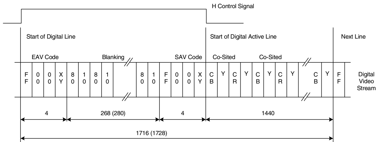
Figure 18-9. LCDIF Interface Signals in ITU-R BT.656 Digital Video Interface Mode
