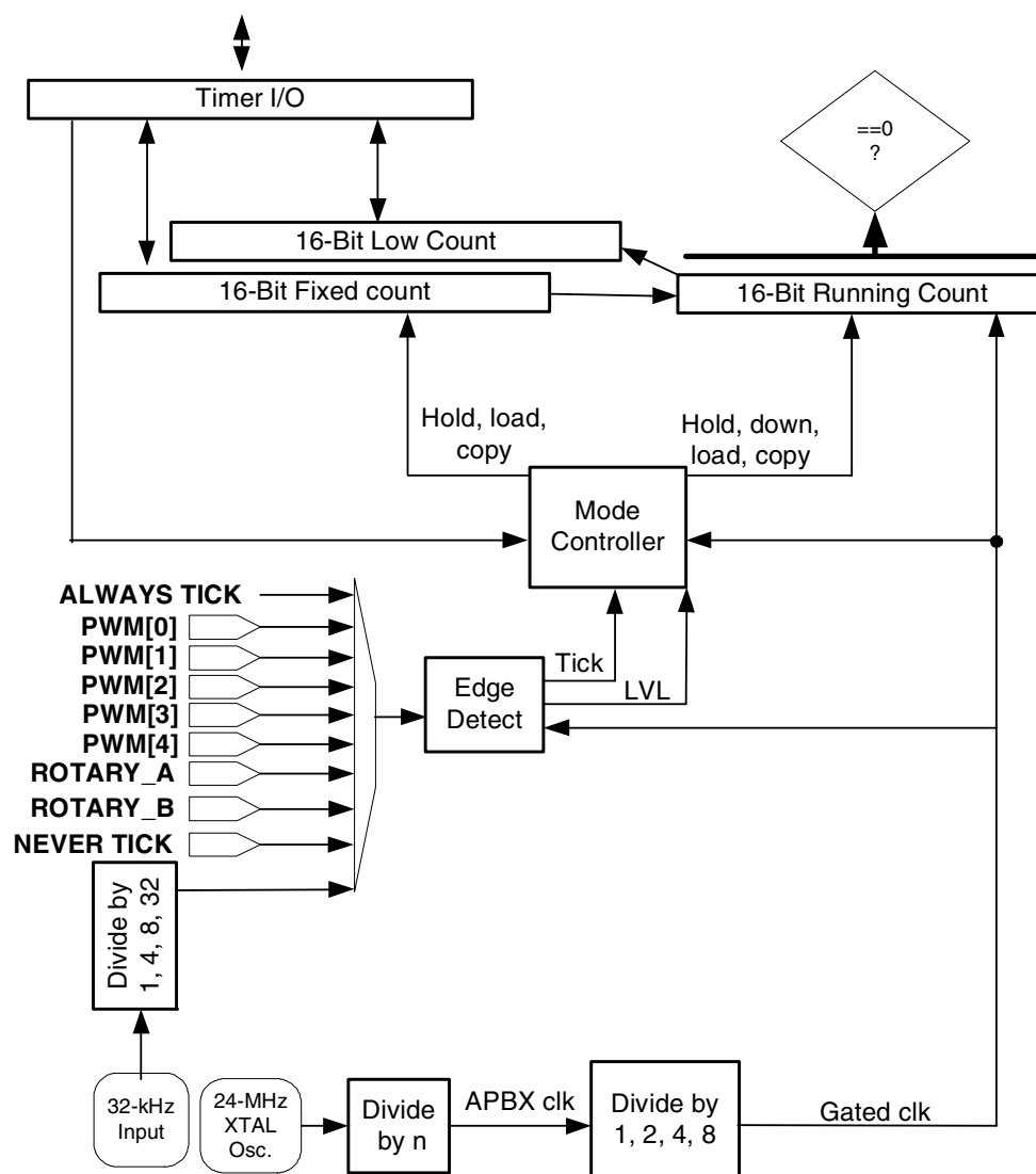
Figure 22-3. Timer 3 Detail
