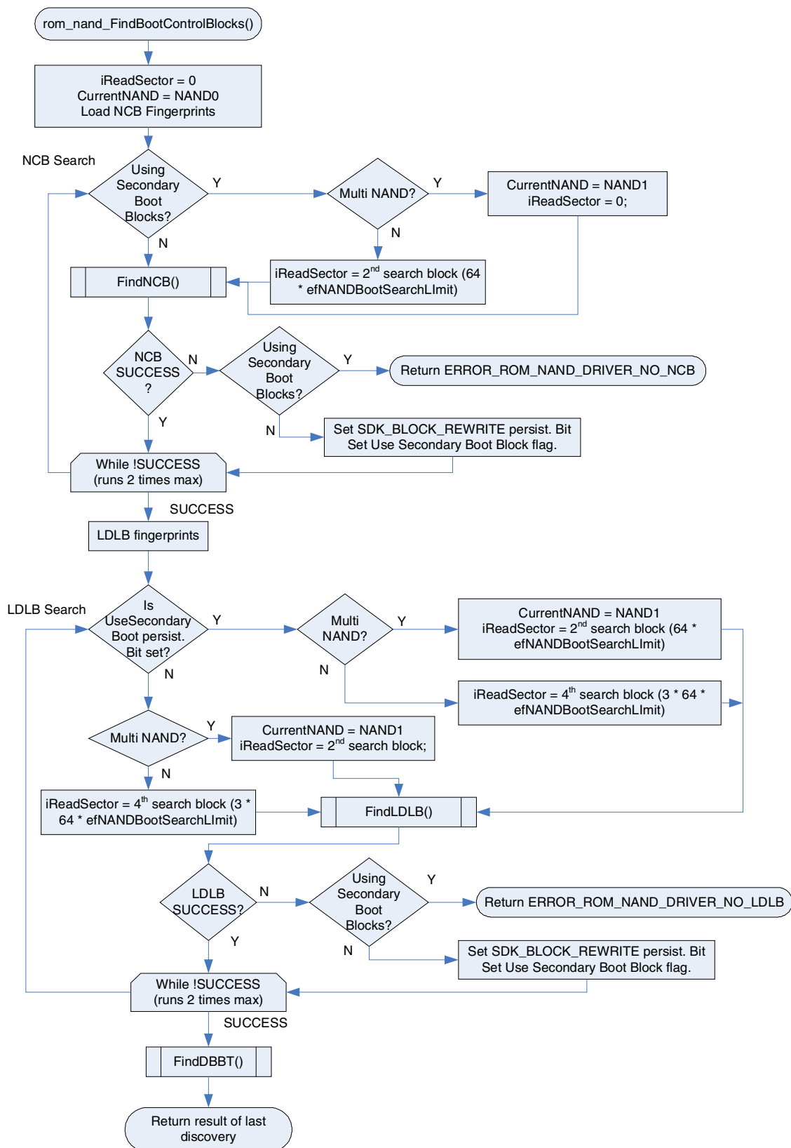
Figure 35-3. FindBootControlBlocks Flowchart
