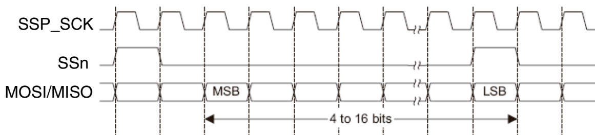
Figure 21-10. Texas Instruments Synchronous Serial Frame Format (Continuous Transfer)
