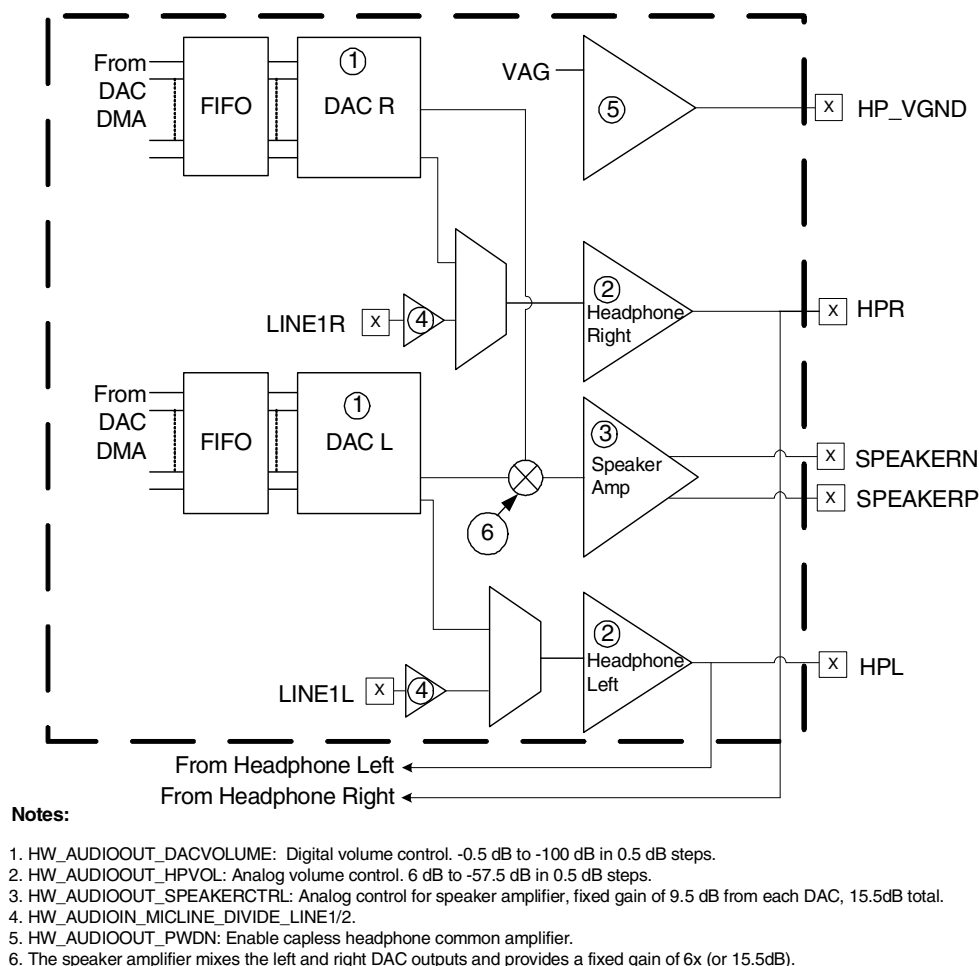
Figure 29-2. AUDIOOUT/DAC Block Diagram
