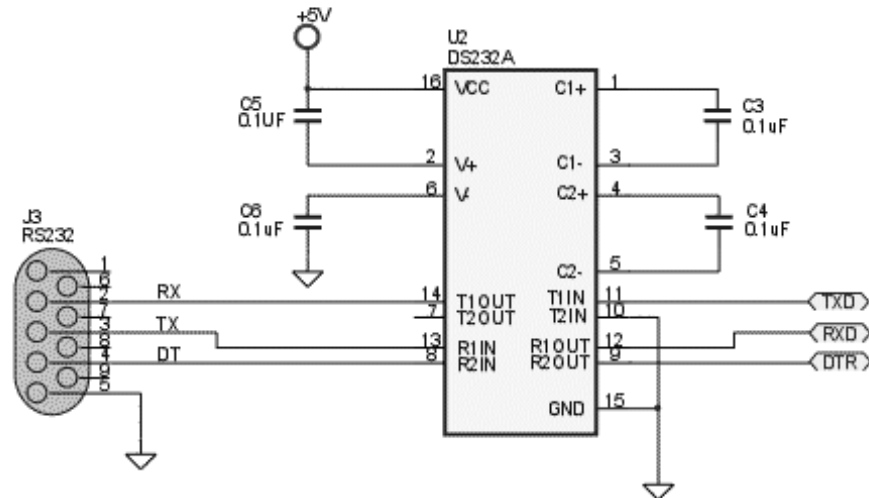
RS232 INTERFACE FOR CHARGER Figure 1
