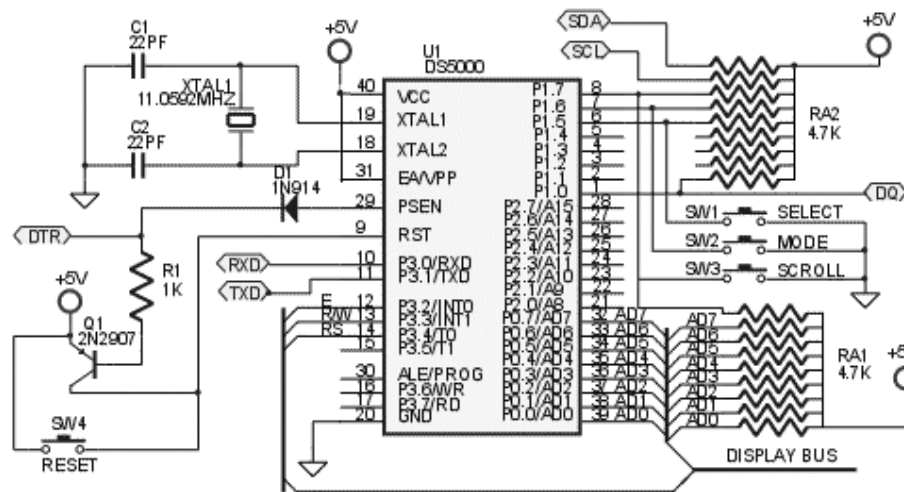
MICROCONTROLLER AND USER PUSHBUTTONS Figure 2
