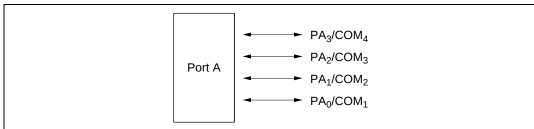
Figure 8.8 Port A Pin Configuration
