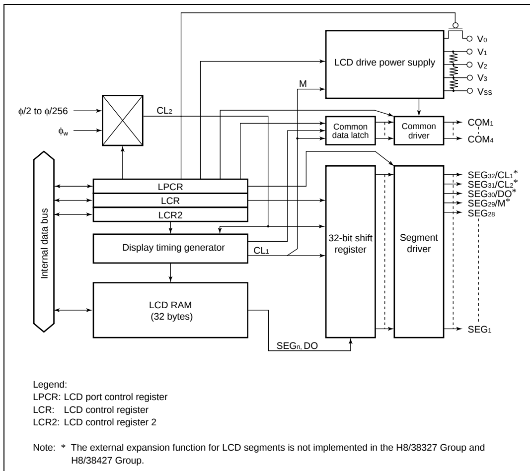
Figure 13.1 shows a block diagram of the LCD controller/driver.
