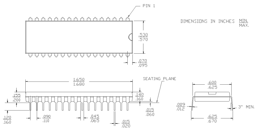
32-Lead (600-Mil) Molded DIP P19
