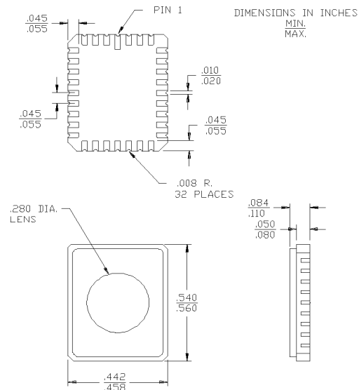
32-Pin Windowed Rectangular Leadless Chjp Carrier Q55
