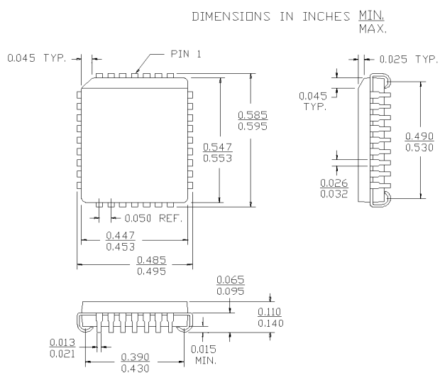
32-Lead Pastic Leaded Chip Carrier J65
