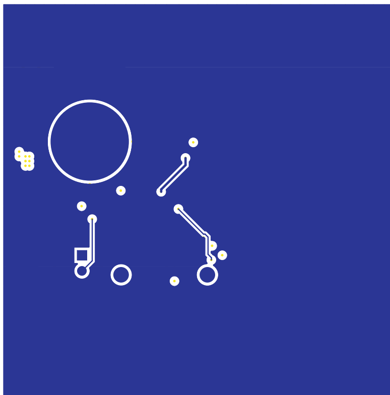
Figure 7. Bottom Layer 4
