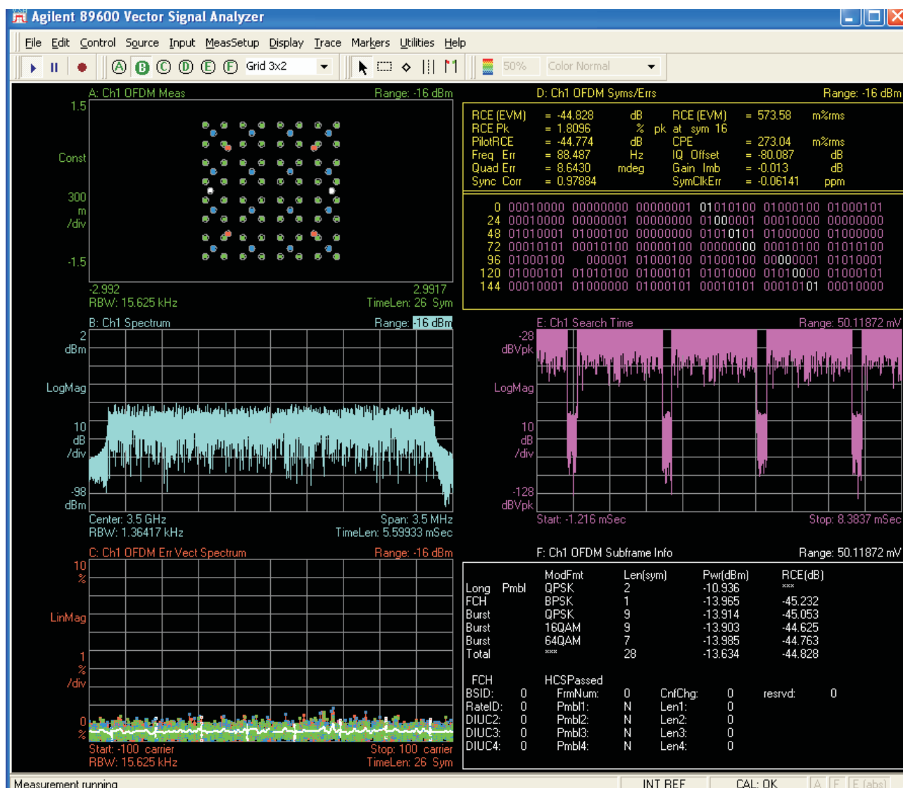
Figure 3. TRF1x22EVM Performance
