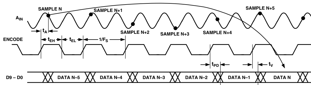
Figure 1. Timing Diagram
