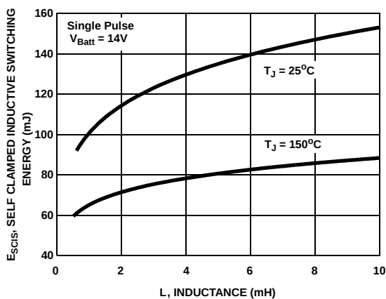
Figure 7. Self Clamped Inductive Switching Energy vs Inductance
