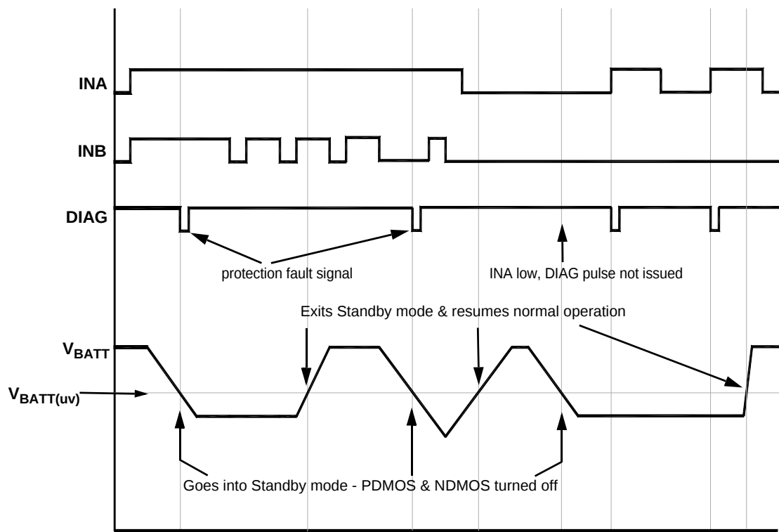
Figure 6. Under-Voltage
