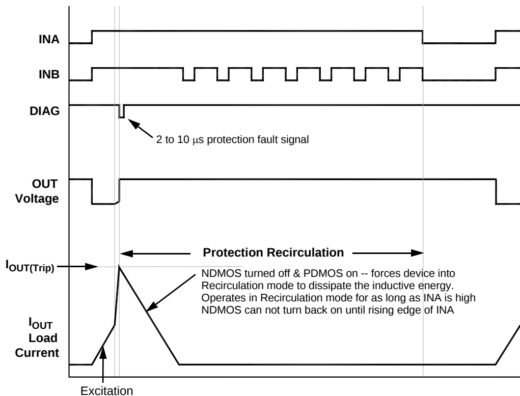
Figure 2. Current Trip
