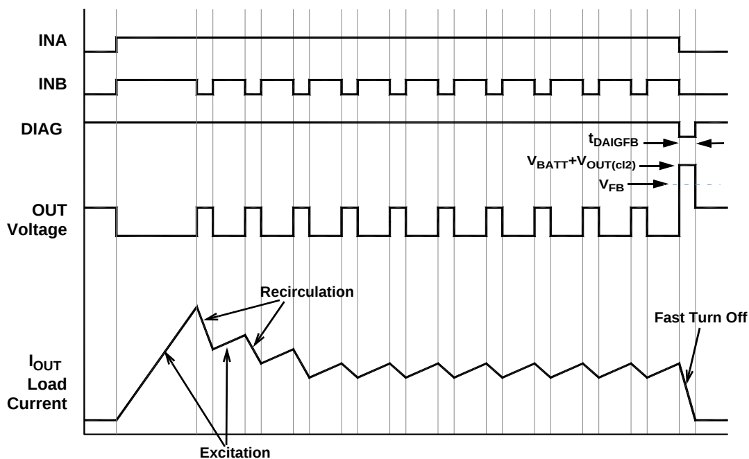
Figure 1. Normal Operation
