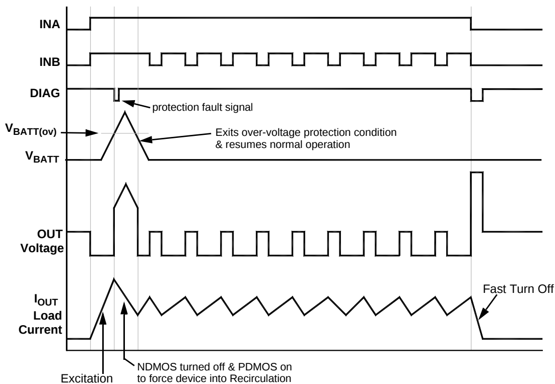
Figure 4. Over-Voltage
