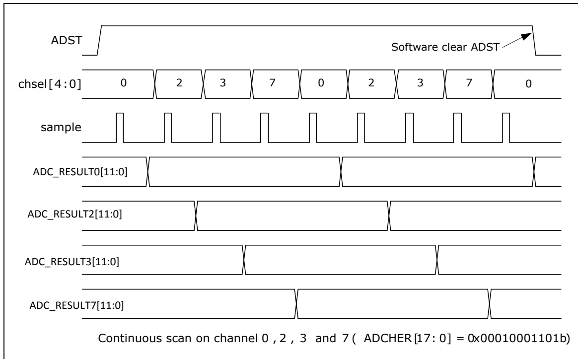
Figure 5-10 ADC Continuous Scan on Enabled Channels Timing Diagram
