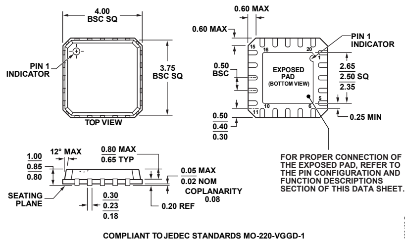
Figure 38. 20-Lead Lead Frame Chip Scale Package [LFCSP_VQ] 4 mm × 4 mm Body, Very Thin Quad (CP-20-4) Dimensions shown in millimeters
