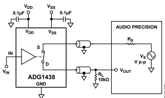
Figure 36. THD + Noise
