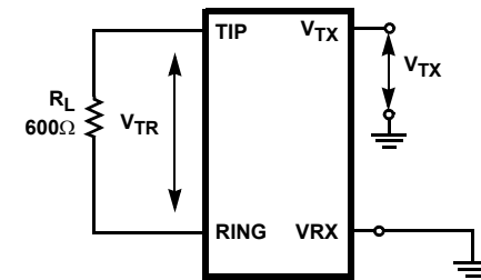
FIGURE 9. IDLE CHANNEL NOISE
