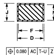
SECTION AE-AE
