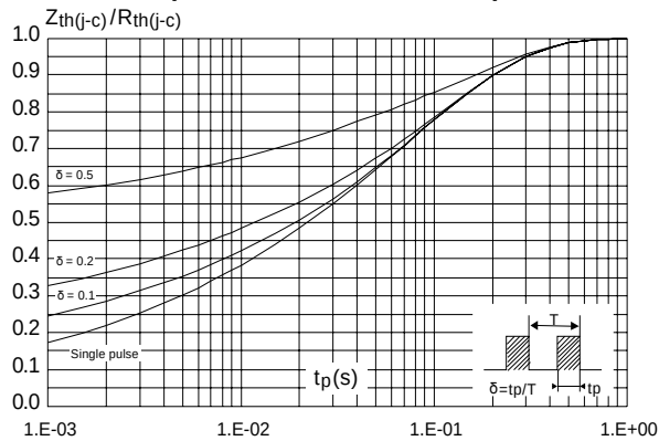
Figure 3: Relative variation of thermal impedance junction to case versus pulse duration (TO-220AC, DPAK, D²PAK)
