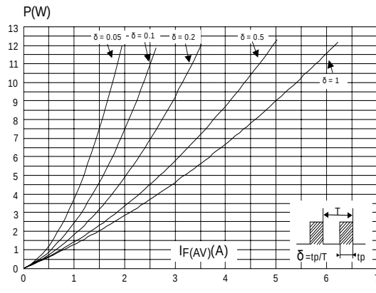
Figure 1: Conduction losses versus average current
