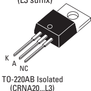
3 Pin Package (L3 suffix)
