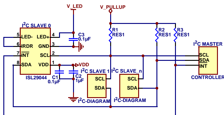
FIGURE 1. TYPICAL APPLICATION
