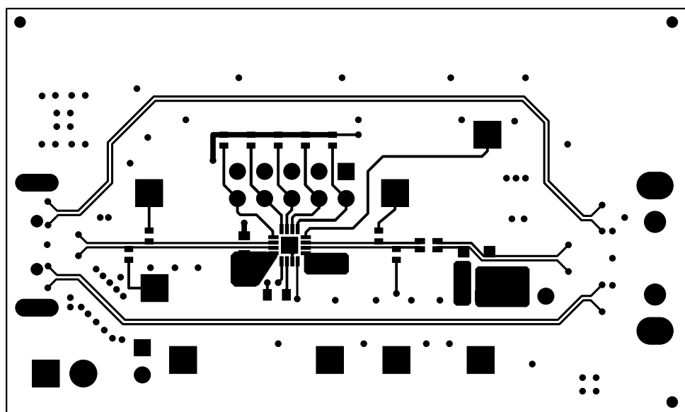
Figure 7. Figure 7. Bottom Side Routing
