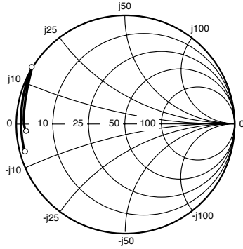
Coordinates in Ohms Frequency in GHz V_D = 3.0\text{ V} , I_D = 600\text{ mA}
