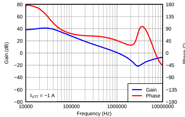
Figure 31. VTT Bode Plot (Sink)
