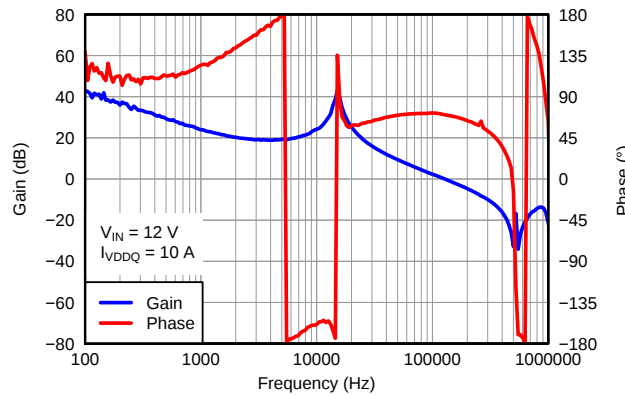
Figure 30. VDDQ Bode Plot
