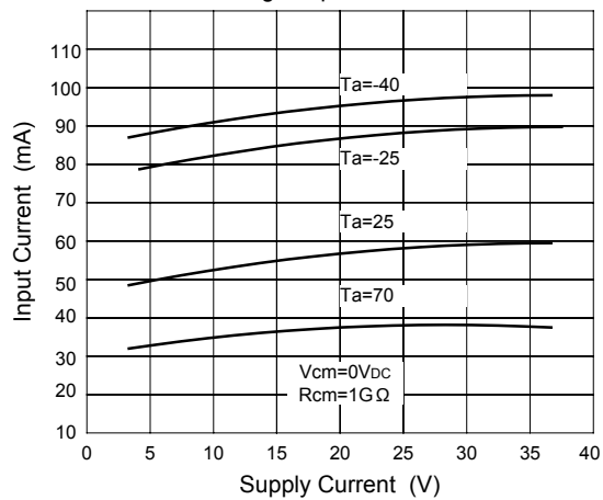
Fig.2 Input Current
