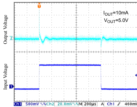
Figure 15. Line Transient
