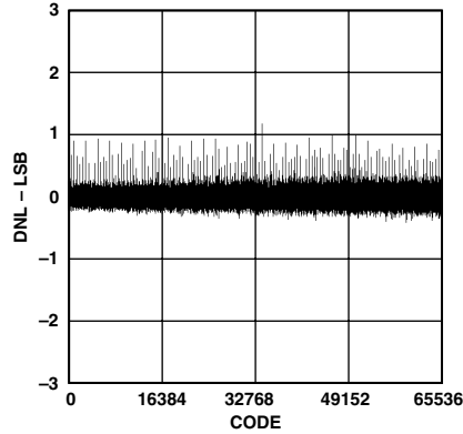
TPC 2. Differential Nonlinearity vs. Code
