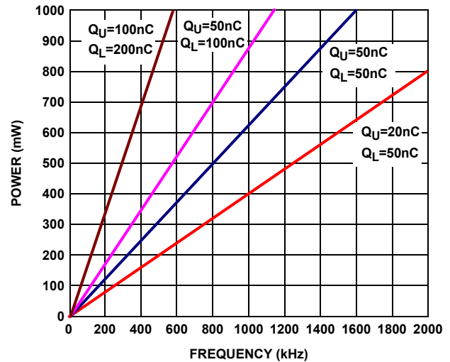
FIGURE 3. POWER DISSIPATION vs FREQUENCY
