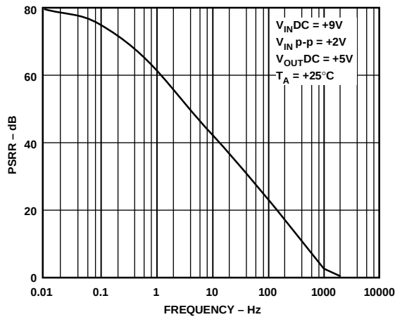
Figure 10. Power Supply Rejection Ratio vs. Frequency
