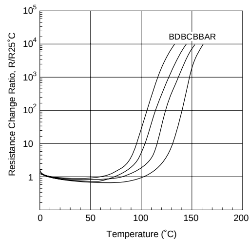
[Resistance-Temperature Characteristic]
