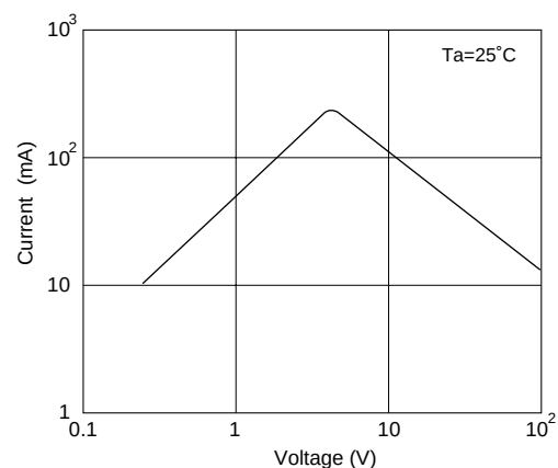
[Current-Voltage Characteristic (Static Characteristic)]
