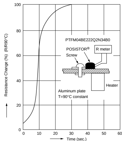
Operating Time of POSISTOR®
