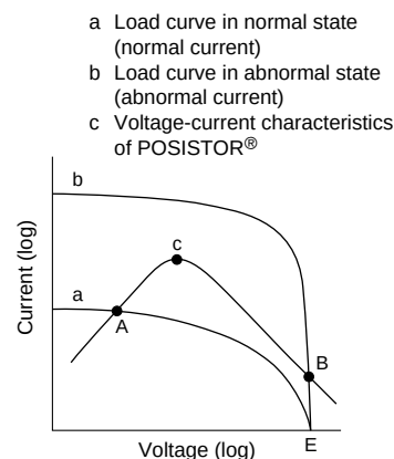
[Load Curve of Circuit and Voltage-current Characteristics of POSISTOR®]
