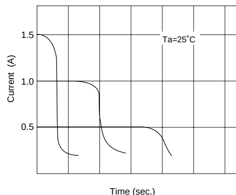
[Current-Time Characteristic (Dynamic Characteristic)]
