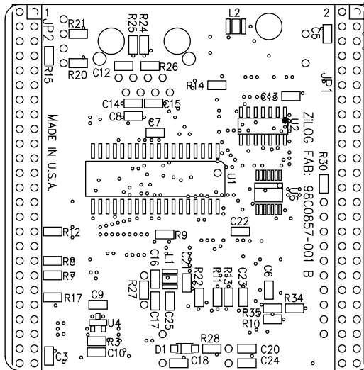
Figure 13. Bottom Layer
