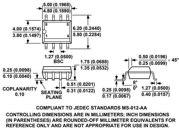
Figure 52. 8-Lead Standard Small Outline Package [SOIC_N] Narrow Body (R-8) Dimensions shown in millimeters and (inches)
