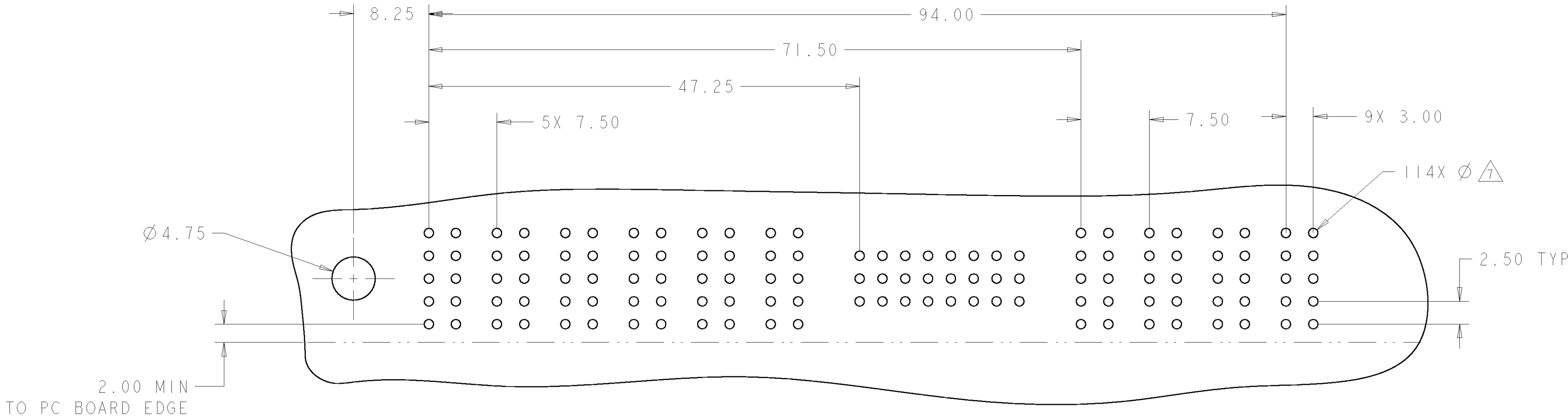
PRINTED CIRCUIT LAYOUT COMPONENT SIDE
