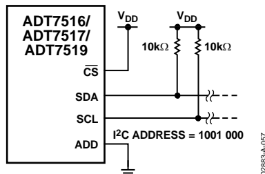
Figure 57. Typical I 2 C Interface Connection
