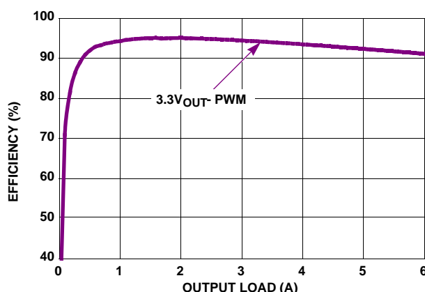
FIGURE 1. EFFICIENCY vs LOAD, 1MHz 5VIN PWM, T_A = +25^\circ\text{C}
