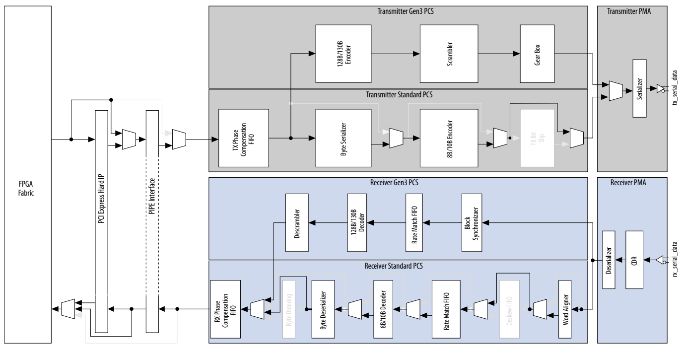
Figure 4-19: Transceiver Channel Datapath for PCIe Gen1/Gen2/Gen3 Configurations
