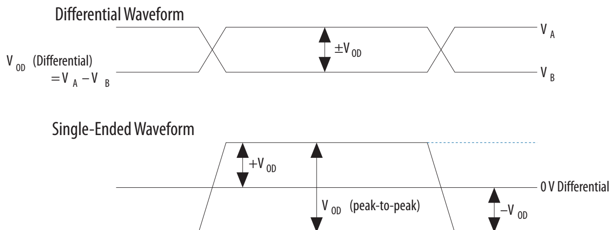
Figure 1-17: VOD (Differential) Signal Level
