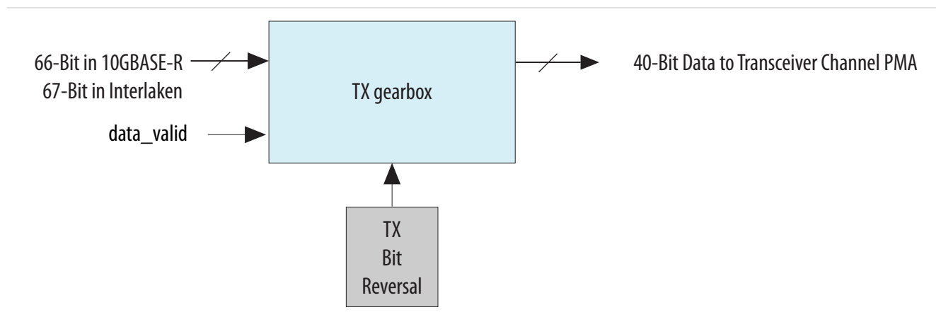
Figure 1-39: Transmitter Gearbox
