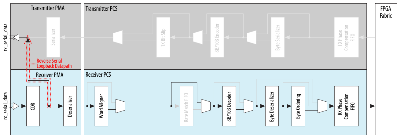
Figure 5-3: Reverse Serial Loopback Datapath
