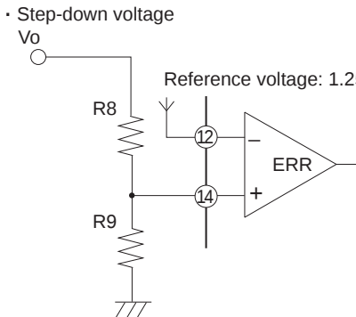
Fig. 15 Step-down voltage
