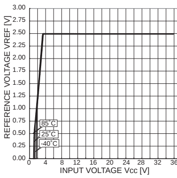
Fig.6 Reference voltage
