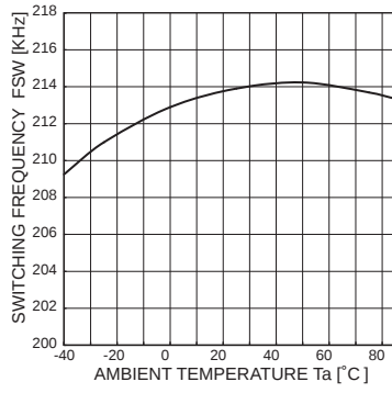
Fig.3 Switching frequency vs. Ambient temperature
