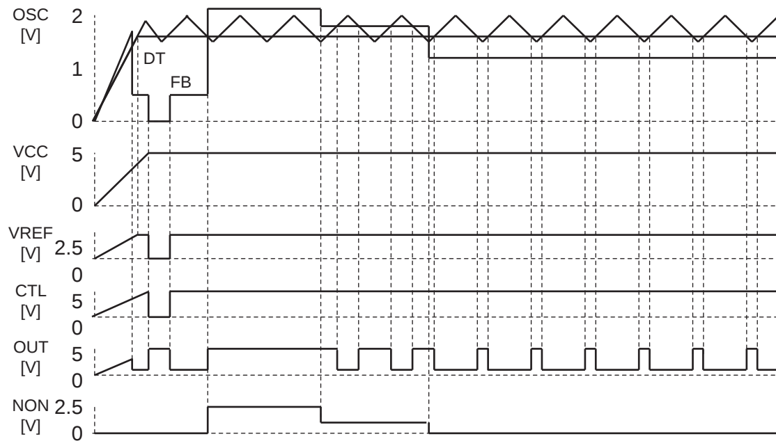
Fig. 13 Basic operation
