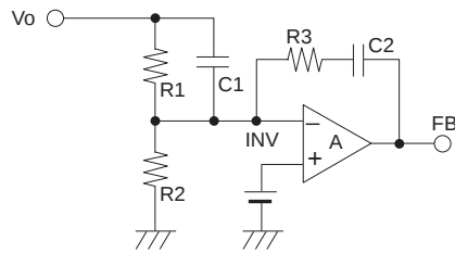
Fig. 25 Typical circuit after secondary compensation circuit
