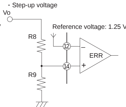
Fig.16 Step-up voltage
