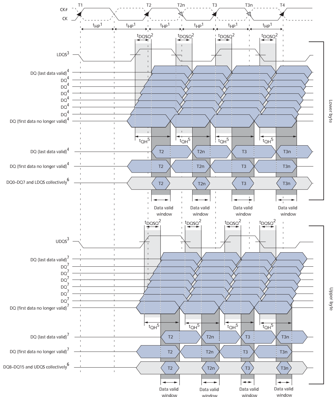
Figure 27: x16 Data Output Timing – t_{DQSQ} , t_{QH} , and Data Valid Window
