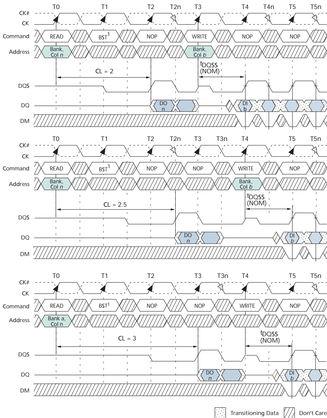
Figure 23: READ-to-WRITE
