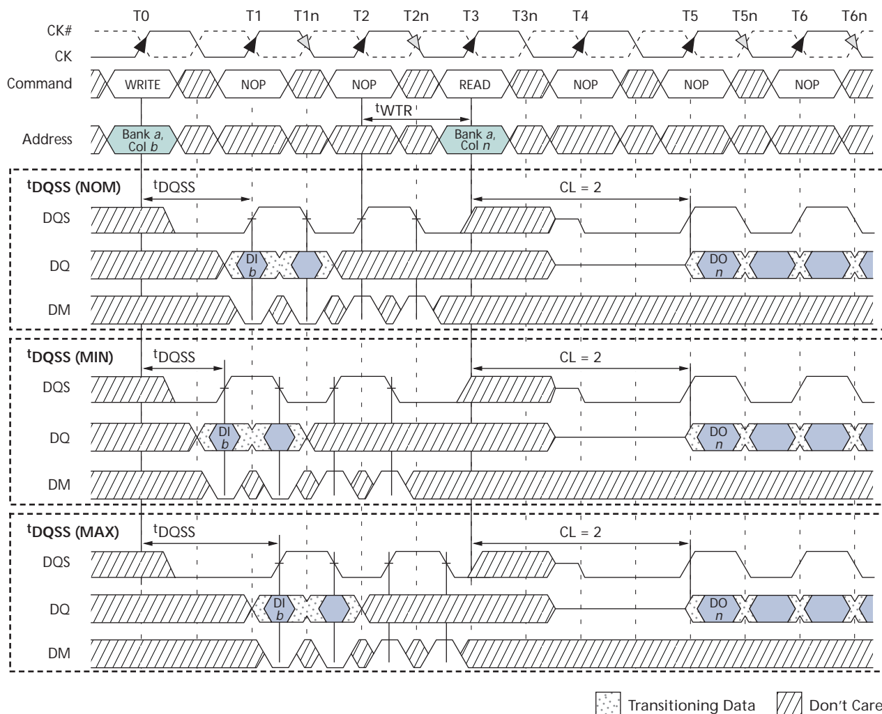
Figure 34: WRITE-to-READ – Interrupting
