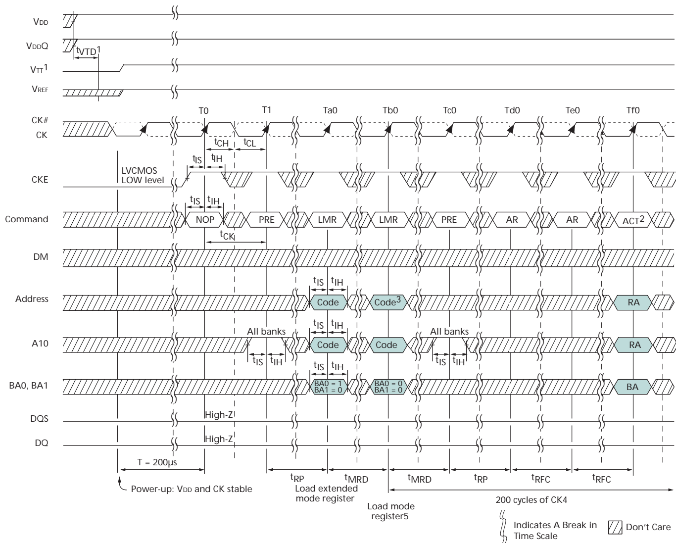
Figure 13: INITIALIZATION Timing Diagram
