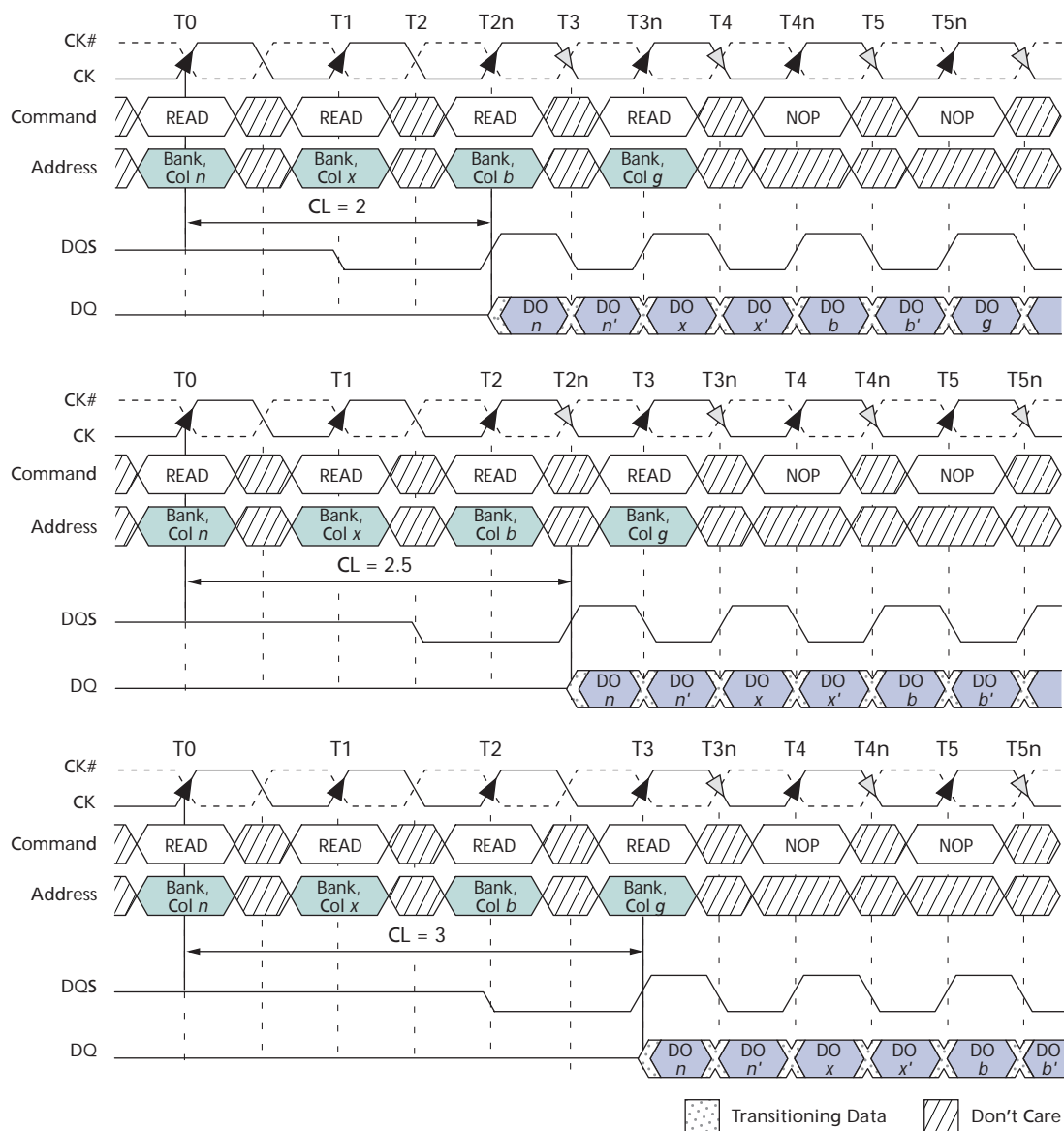
Figure 21: Random READ Accesses
