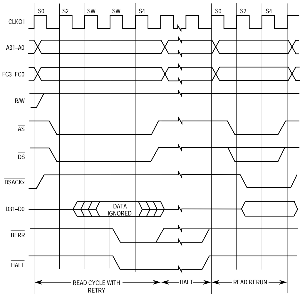
Figure 4-31. Retry Sequence
