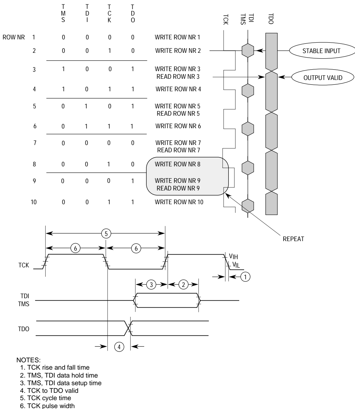
Figure 9-26. Bit Banging of Boundary Scan Pattern
