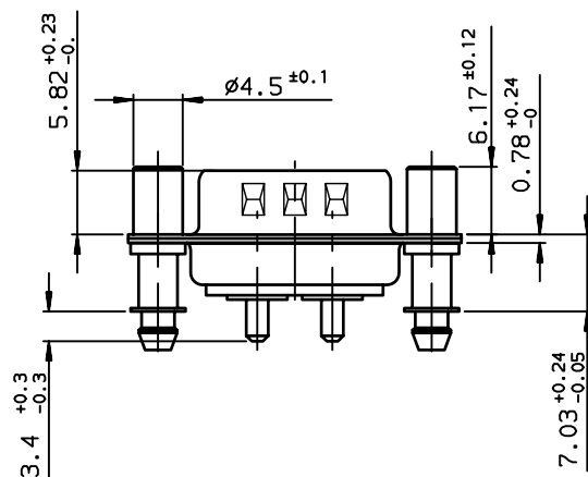
LAYOUT DIMENSIONS (after plating) CONNECTOR SIDE VIEW
