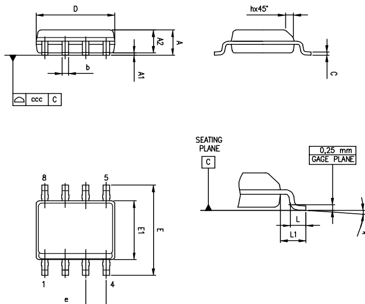
Figure 35. SO8 package outline
