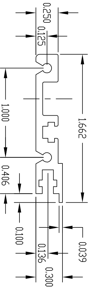
CROSS-SECTIONAL DETAIL
