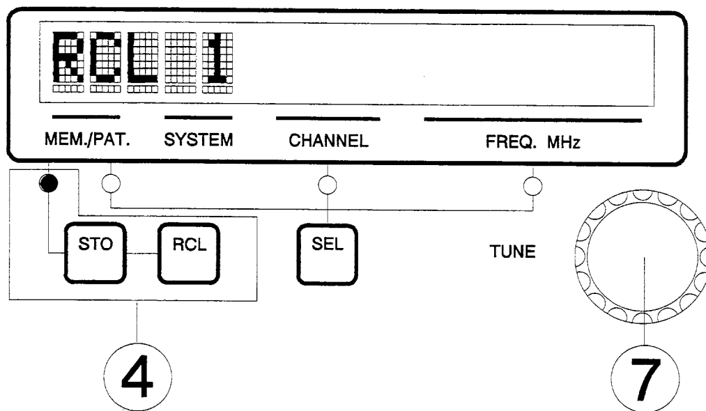
Figure 4.– Selection of TV standard and memory.
