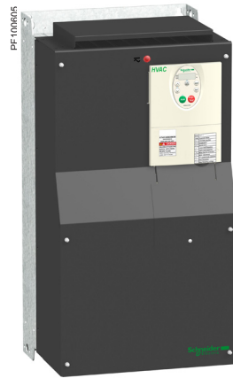
ATV 212HD55N4 EMC plate not mounted
