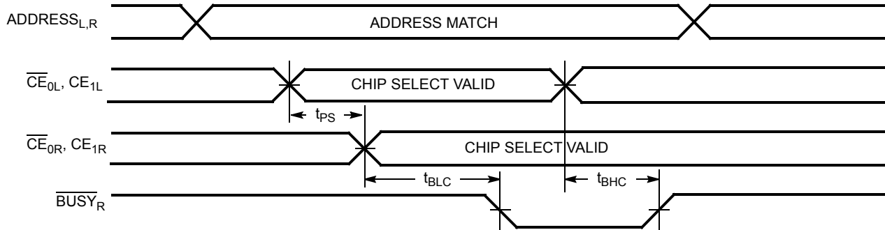
Figure 13. Busy Timing Diagram No. 1 ( \overline{CE} Arbitration) [54]
