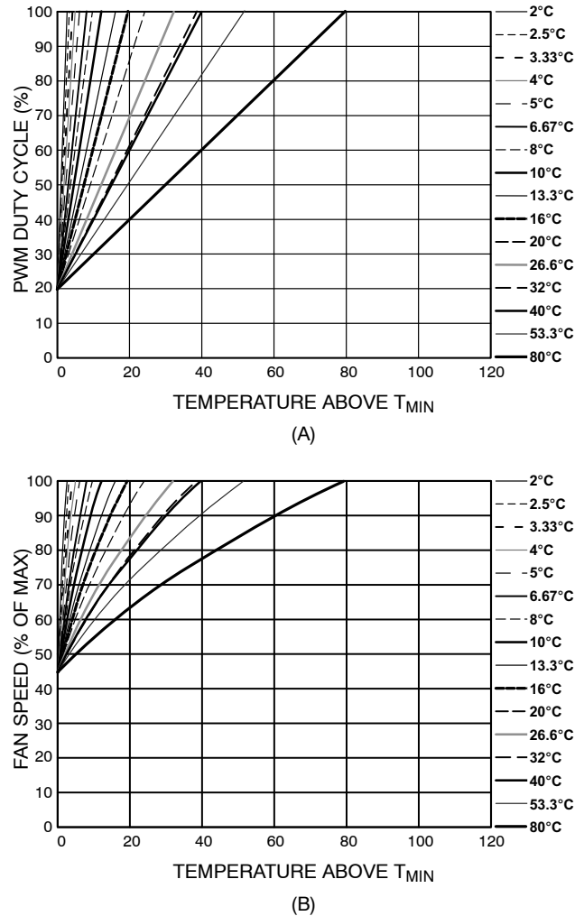
Figure 58. T_{\text{RANGE}} and % Fan Speed Slopes with \text{PWM}_{\text{MIN}} = 20\%
