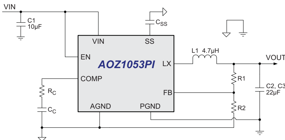
Figure 1. 3.3V, 5A Synchronous Buck Regulator, Fs = 450kHz
