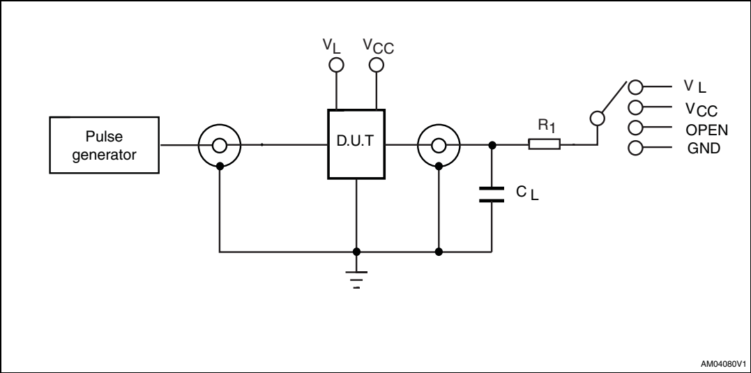
Figure 5. Test circuit
