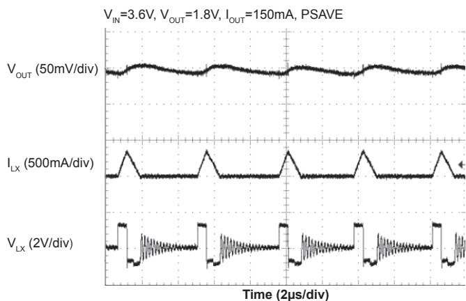
PSAVE Operation
