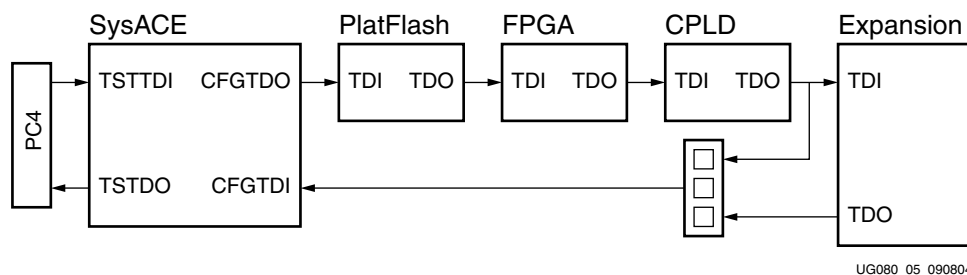
Figure 5: JTAG Chain
