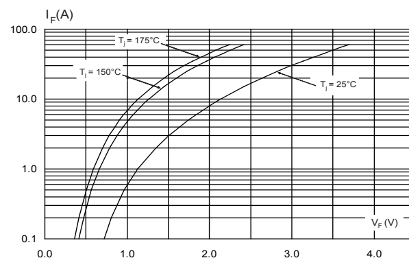
Figure 6. Forward voltage drop versus forward current (maximum values)
