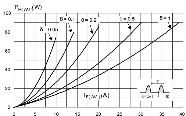
Figure 4. Average forward power dissipation versus average forward current (sinusoidal waveform, DO-247 LL)
