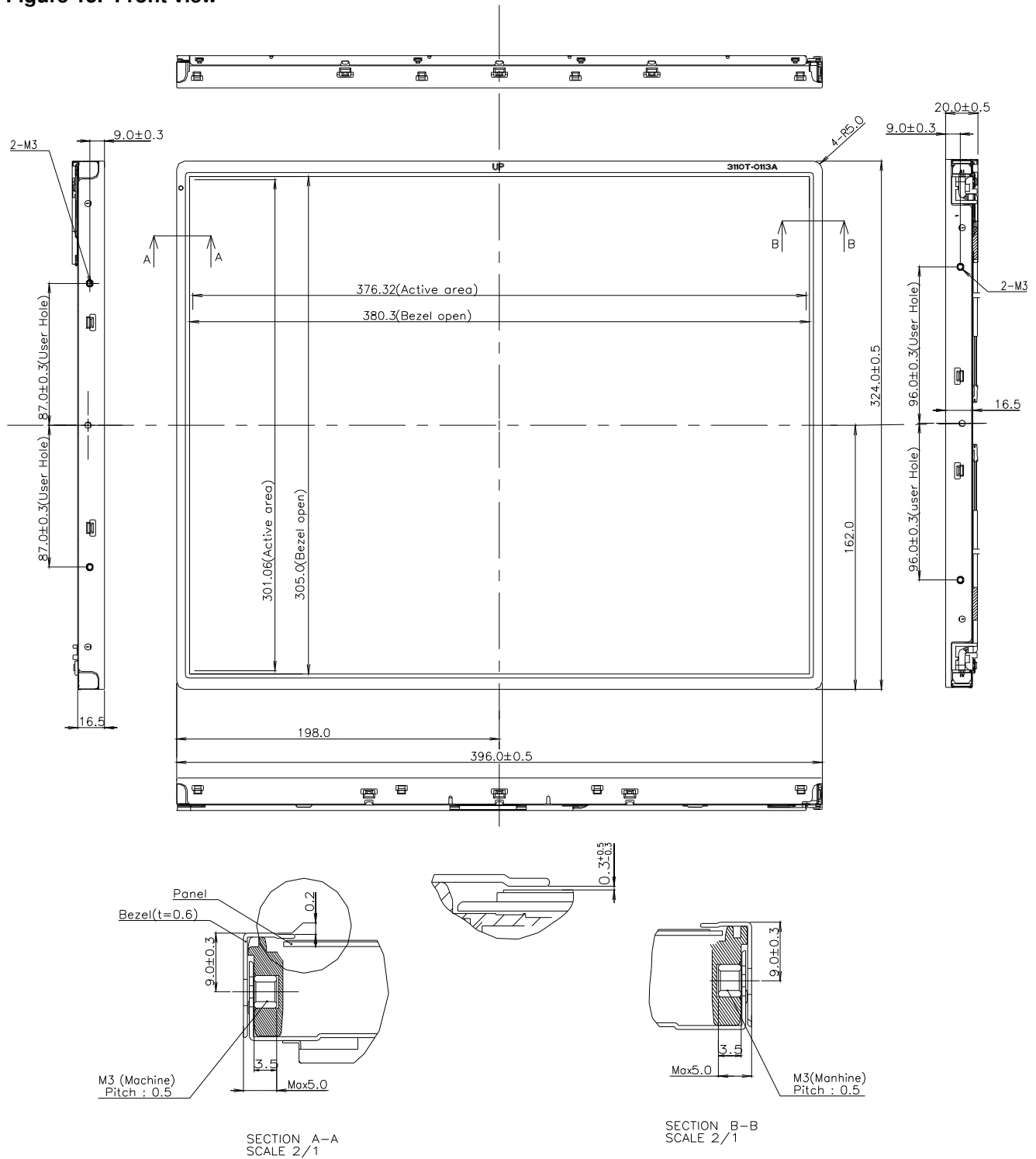
Figure 15. Front view
