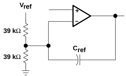
Test Circuit
