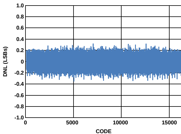
FIGURE 13. DIFFERENTIAL NONLINEARITY (125MSPS)
